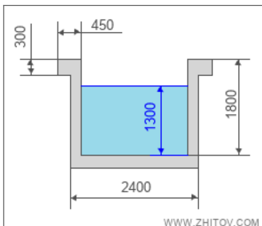
Basin dimensions - front view
