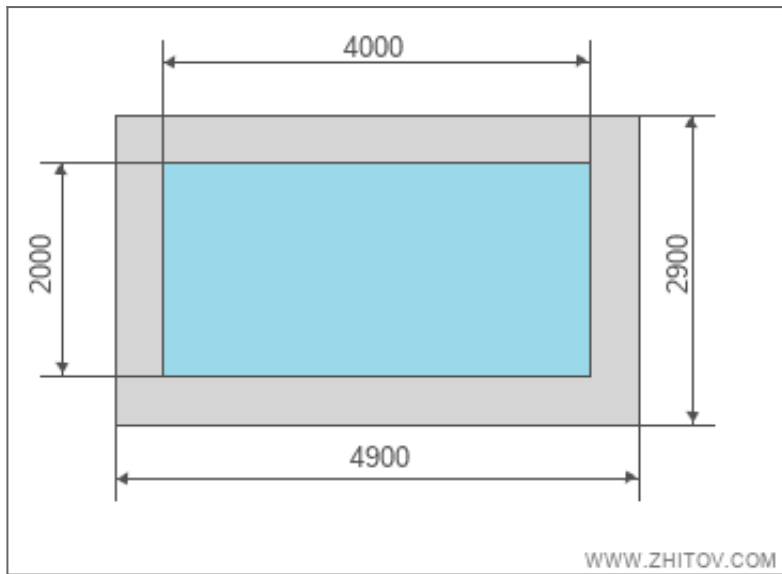
Basin dimensions - Top view
