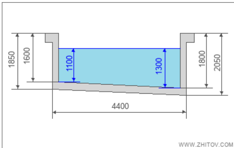
Basin dimensions - side view
